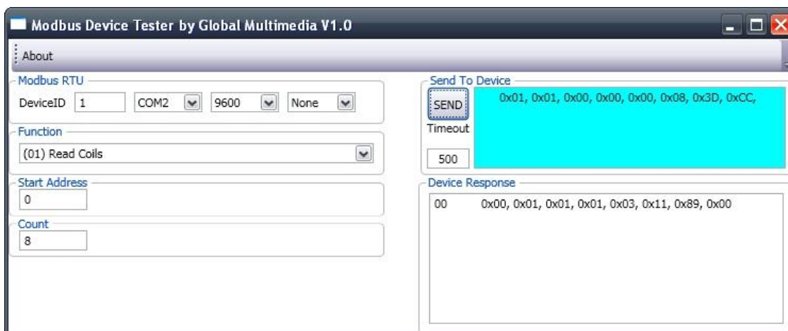
Figure 13 - Modbus Response Data From CSC400 with Line Polarization OFF
