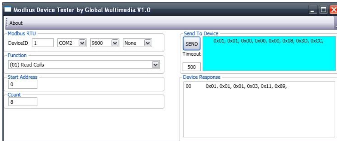
Figure 12 - Modbus Response Data From CSC400 with Line Polarization ON
